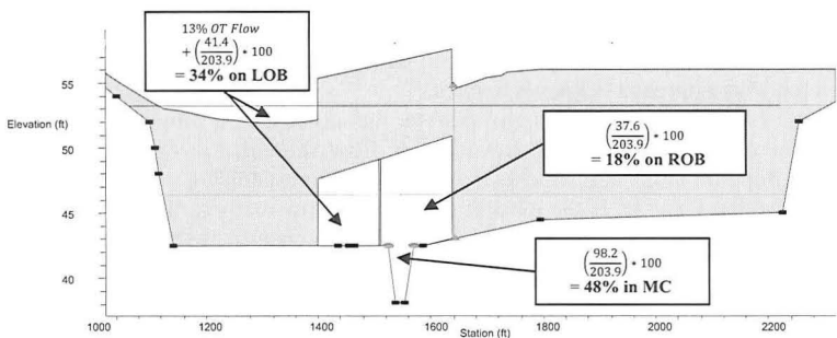
Figure 1 - Bridge Section with Target Values
