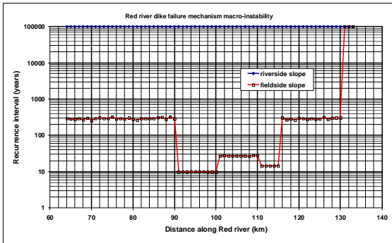
Figure 10. Recurrence intervals for mechanism macro-instability along Red River
