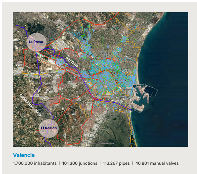
Figure 1 | Characteristics of the WSDN of Valencia and Eindhoven.
