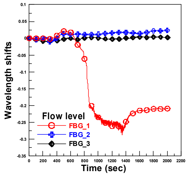
Fig.7 Test results of flow level __Model-II
