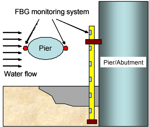
Fig. 2 The FBG scour monitoring system --Model II
