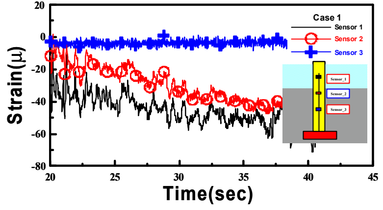
Fig. 3 Model I-- sensor_1 emerges out the sediment
