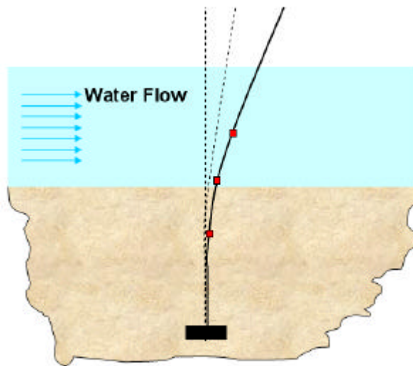
Fig. 1 The FBG scour monitoring system --Model I
