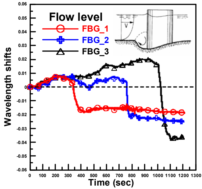
Fig.8 Test results of flow level __Model-II-case2
