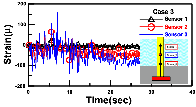
Fig. 5 Model I-- sensor_3 emerges out the sediment
