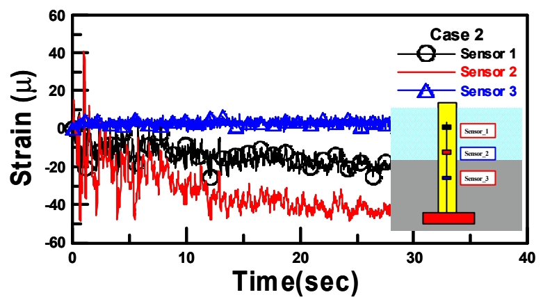
Fig. 4 Model I-- sensor_2 emerges out the sediment
