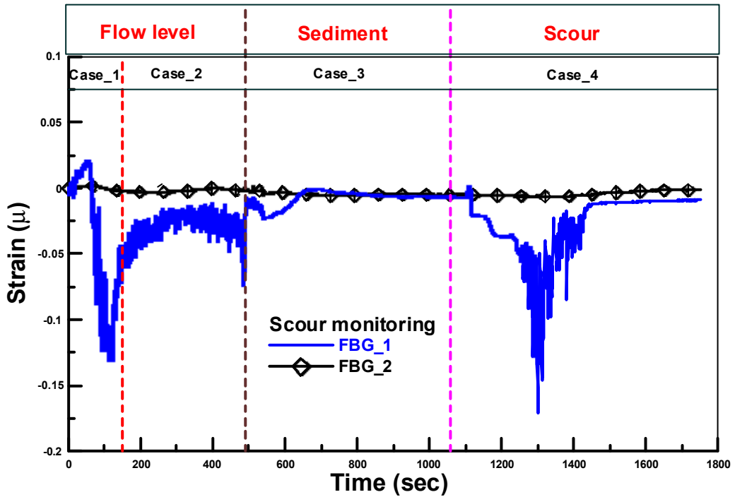
Fig. 9 Scouring test of Model II
