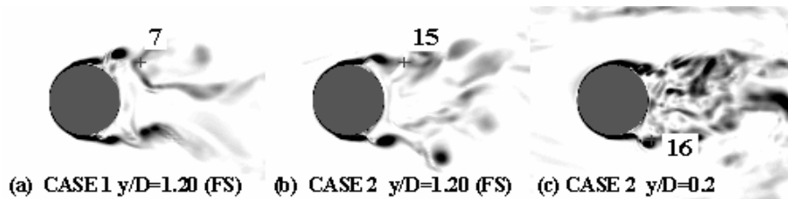
Figure 7. Instantaneous vorticity magnitude contours |\omega_z|D/U at the free surface ( y/D = 1.2 ) and close to the bed ( y/D = 0.2 ) showing the vortical structures in the detached shear layers.
