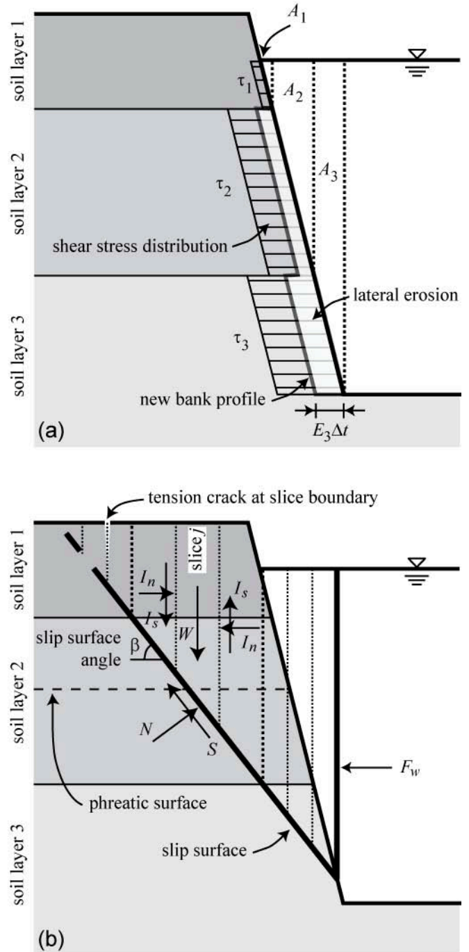
Figure 1. Assessment of streambank erosion processes. (a) Fluvial erosion: the shown shear stress distribution is calculated using the vertical area method. (b) Mass failure: failure block configuration and forces acting on slice j , where I_{ns} = interslice normal and shear force, N = normal force on slice base, S = mobilized shear force on slice base, W = weight of slice, F_w = hydrostatic force exerted by the surface water on the vertical part of the slip surface, and \beta = failure plane angle.
