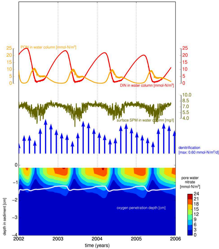
Figure 3. The results of the fully coupled 1d system at Helgoland. The SPM, PON, and DIN concentrations are given for the center of the water column, denitrification fluxes are integrated over the sediment depth and the white line in the lower panel shows the oxygen penetration depth, at which the oxygen concentrations are below 0.1 \text{ mmol-O}_2 / \text{m}^3 .
