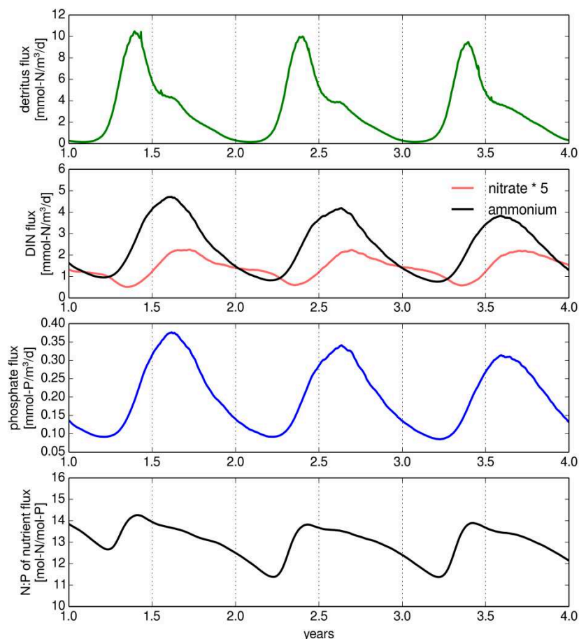
Figure 5. Nutrient fluxes between sediment and water column. The detritus flux is directed into the sediment, whereas the DIN and phosphate flux is directed into the water column. The N:P ratios are well below the Redfield ratio of 16 molN:molP.
