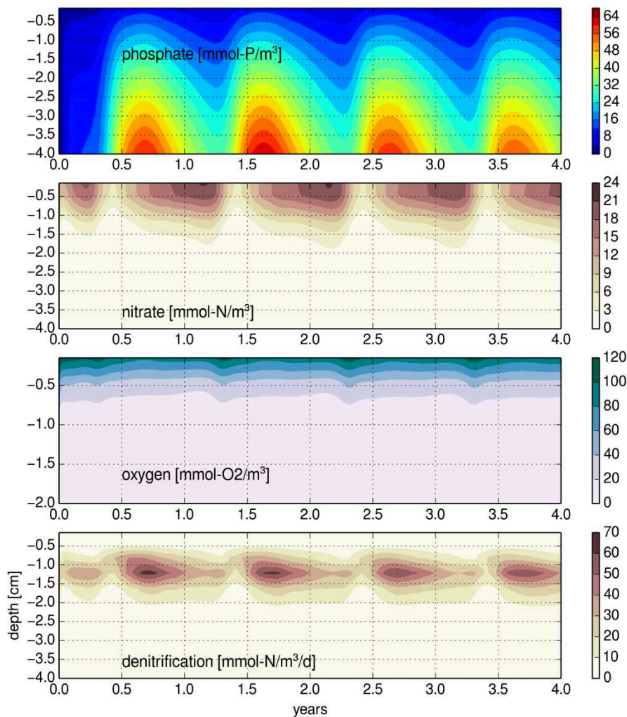
Figure 4. The vertical profiles of phosphate, nitrate, oxygen and the denitrification rate over time. The vertical axis always shows depth below the sediment surface.
