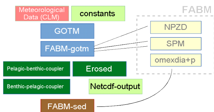
Figure 1. The schematic setup of MOSSCO components for the coupled simulations. The coloured boxes represent ESMF components that exchange fields with standard names.
