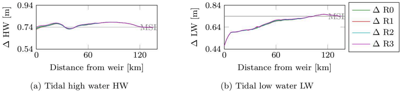
Figure 6. Changes in tidal characteristics along the main river channel for different model roughness distributions for the MSLR scenario.
