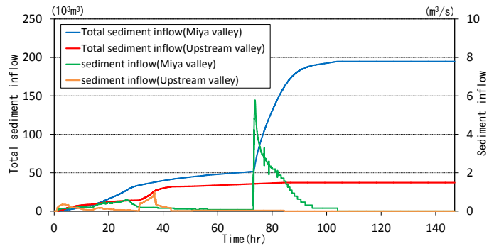
Figure 8. Calculated sediment inflow from mountain streams.
