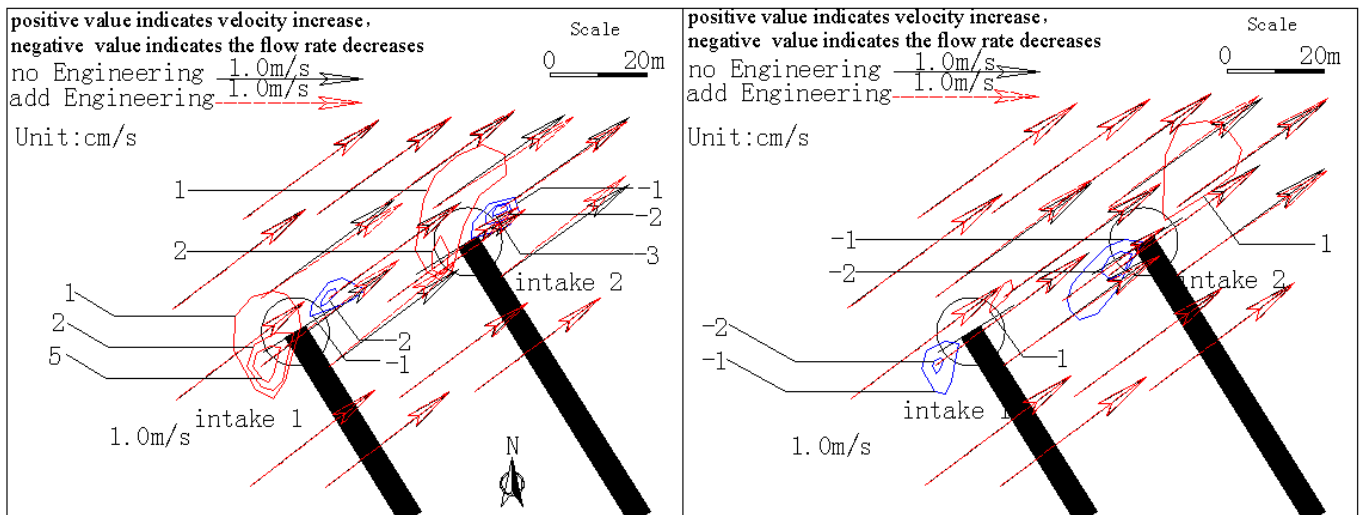
Figure 3. Velocity variation around the intake of design 1.
