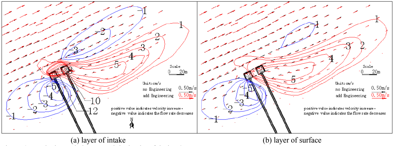
Figure 4. Velocity variation around the intake of design 2.
