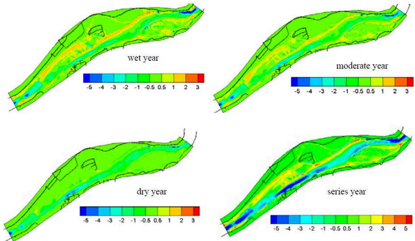
Figure 6. The erosion-deposition distribution in different conditions.
