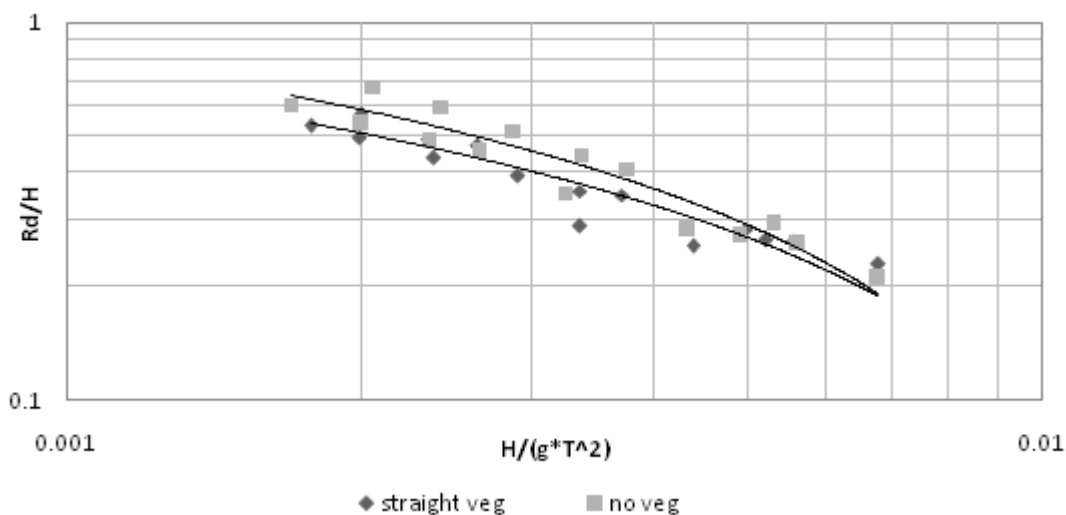
Figure 4. Variation of Rd/H with H/gT^2 .
