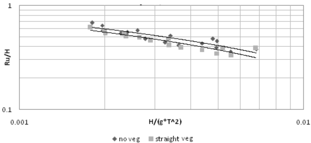
Figure 3. Variation of Ru/H with H/gT^2 .
