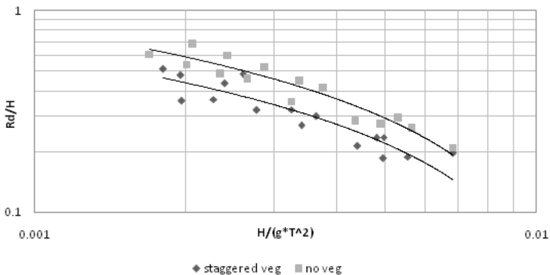
Figure 6. Variation of R_d/H with H_o/gT^2 .
