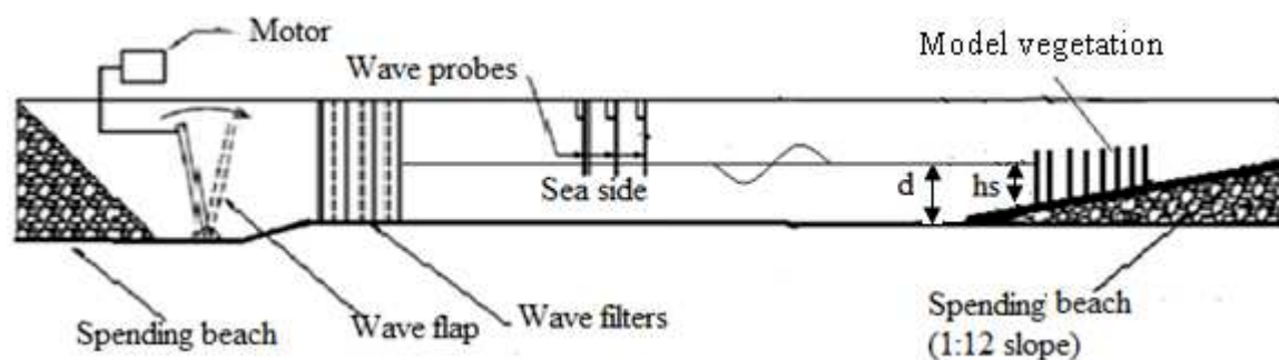
Figure 1. Details of experimental setup.
