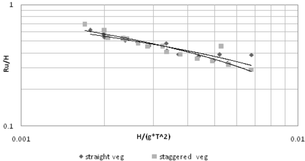
Figure 7. Variation of R_u/H with H_0/gT^2 .
