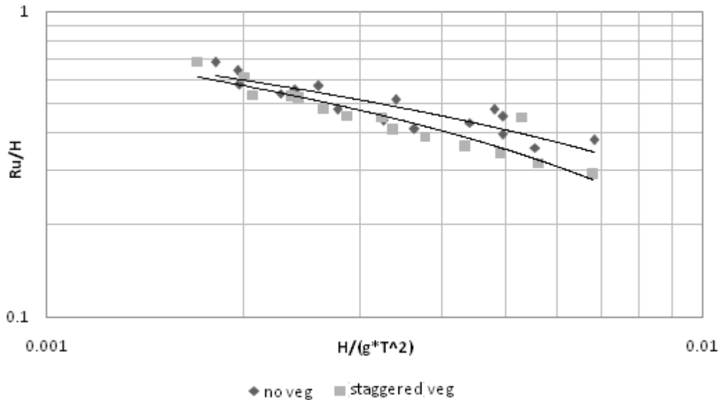
Figure 5. Variation of R_u/H with H_o/gT^2 .
