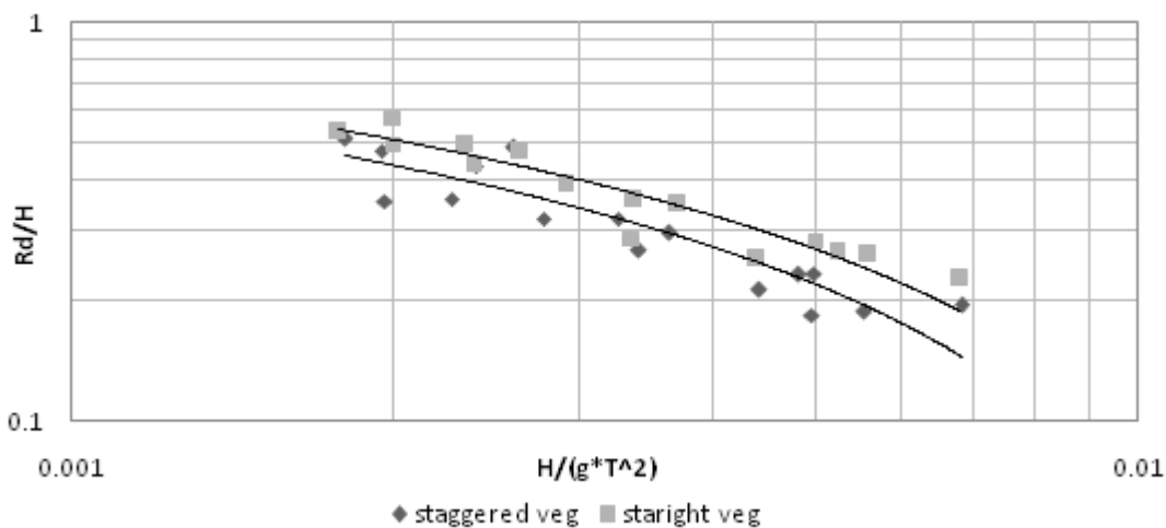
Figure 8. Variation of R_d/H with H_0/gT^2 .
