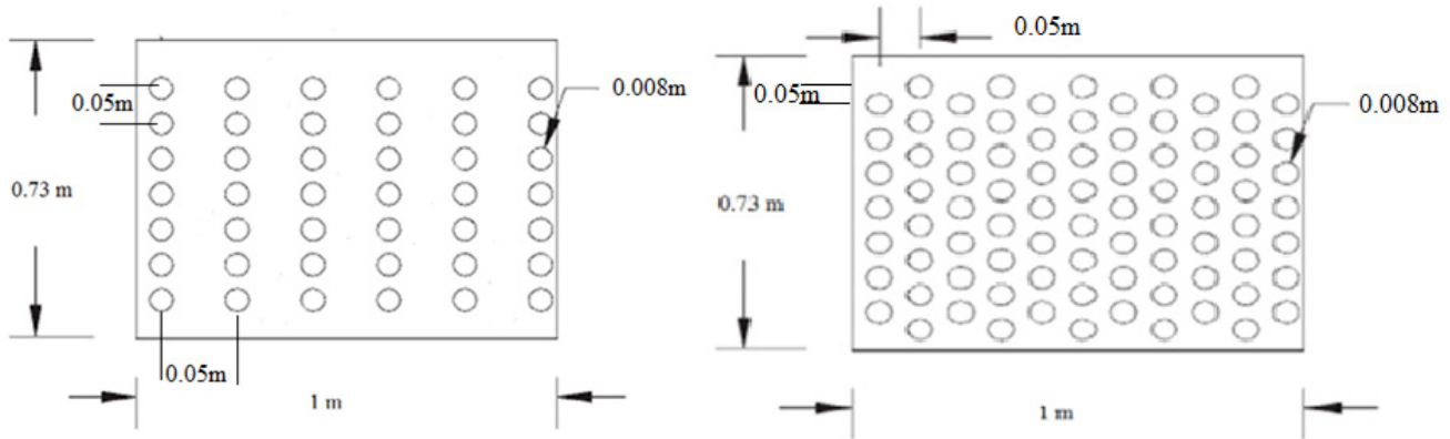
Figure 2. Schematic representation of straight and staggered arrangement of model vegetation.
