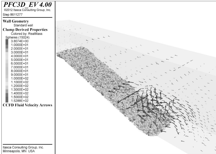
Figure 4. Rip-rap generated in PFC, coupled computation with wave impact.
