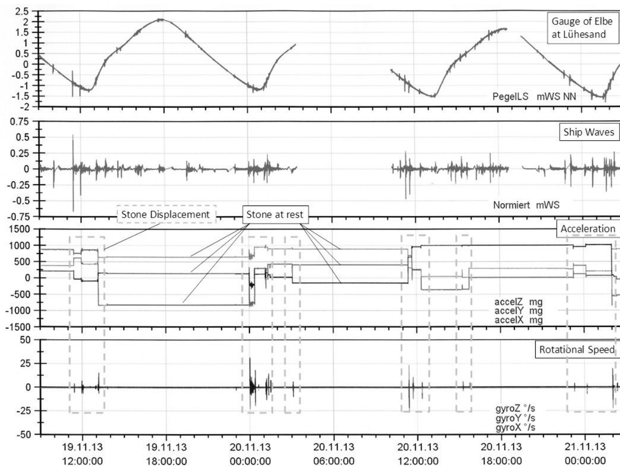
Figure 7. Example of measurements with equipped armourstones in field test.
