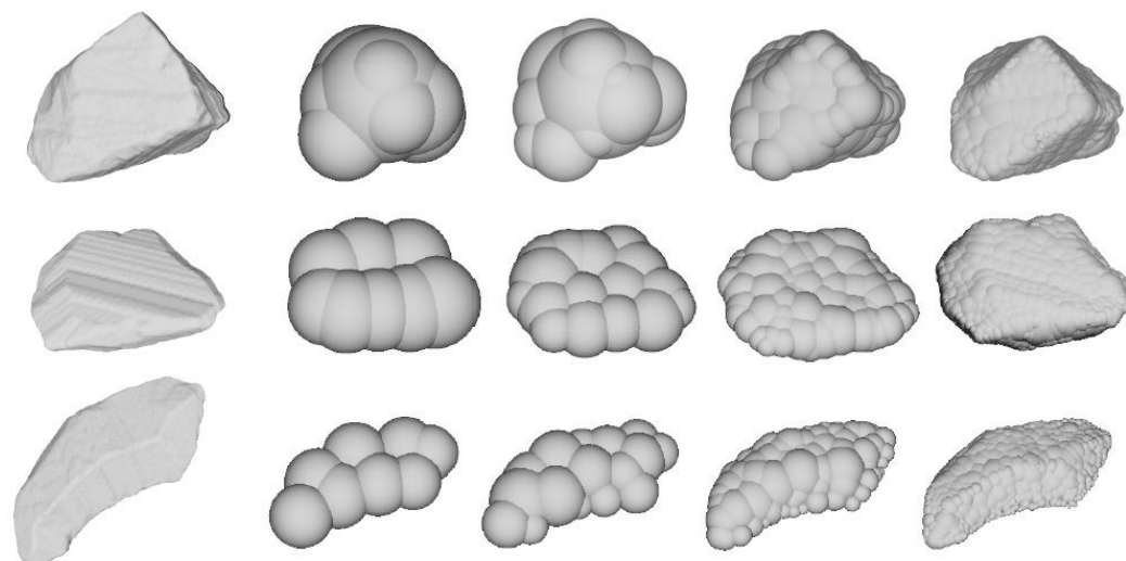
Figure 2. Representation of armourstones as clumps (Yuan 2012).
