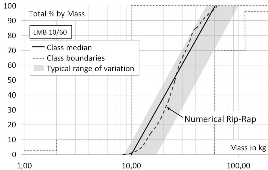
Figure 3. Typical range of variation of cumulative curve for armourstones class LMB 10/60 (BAW 2008), cumulative curve of corresponding numerical rip-rap.
