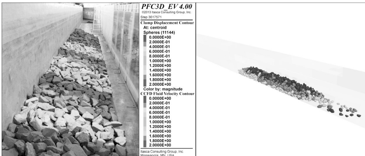
Figure 6. Rip-rap section in hydraulic flume and numerical simulation of physical model tests.
