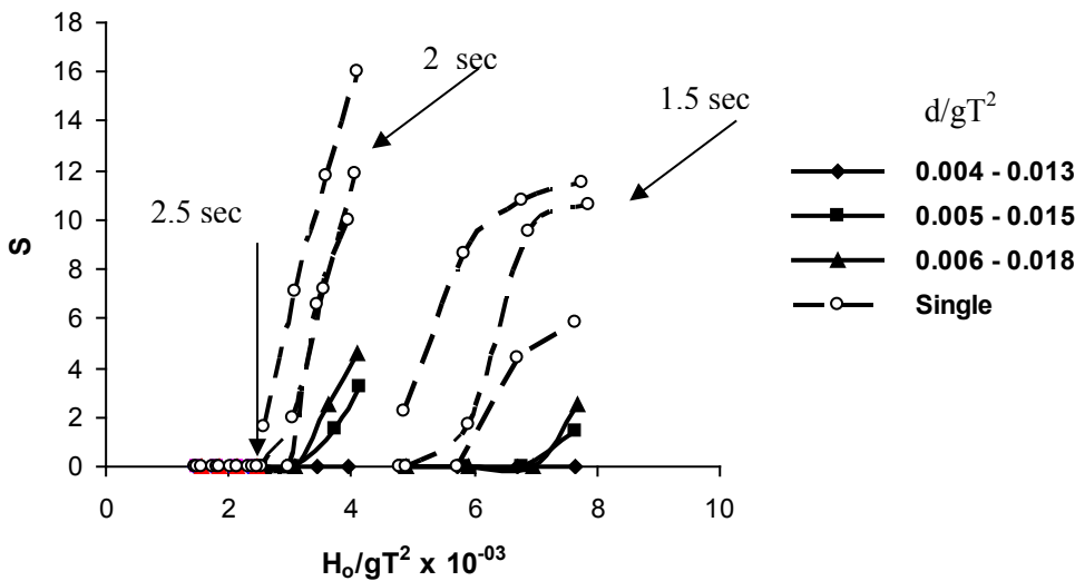
Figure 5. Variation of S with H_o/gT^2 .
