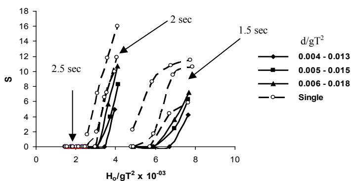
Figure 9. Variation of S with H_o/gT^2 .
