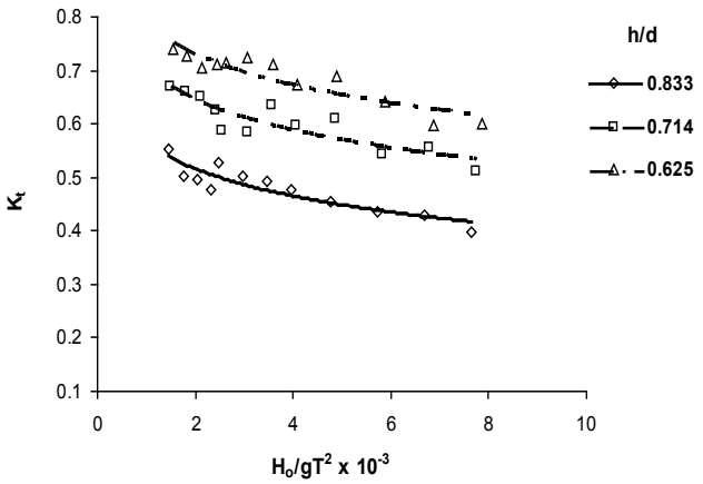
Figure 6. Variation of K_t with H_o/gT^2
