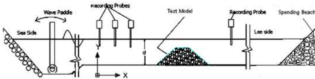
Figure 1. Details of experimental setup.
