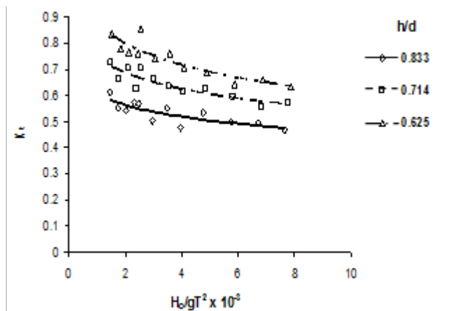
Figure 8. Variation of K_t with H_o/gT^2
