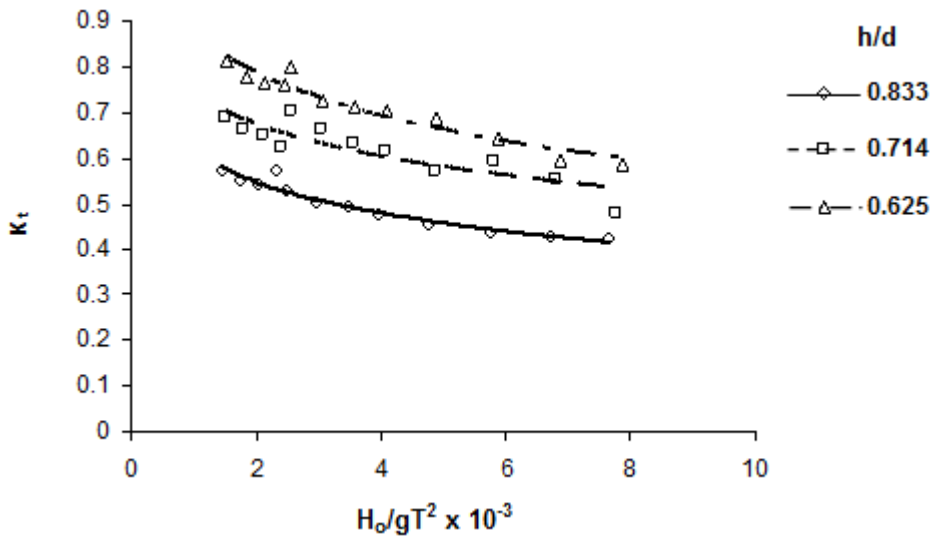
Figure 4. Variation of K_t with H_o/gT^2 .
