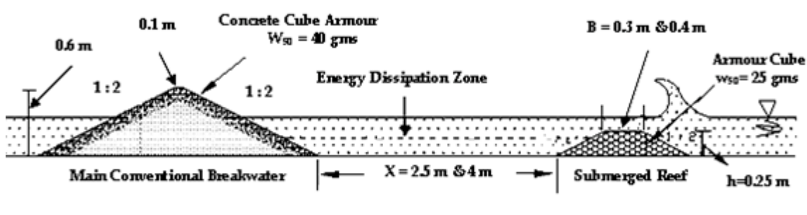
Figure 2. Details of test model of tandem breakwater.
