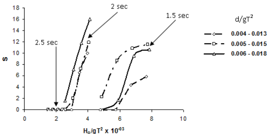
Figure 3. Variation of S with H_o/gT^2 .
