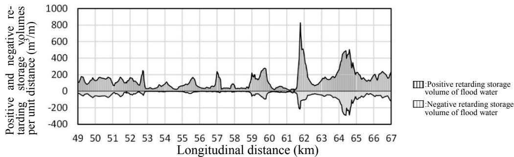
Figure 8. Longitudinal distribution of positive and negative retarding storage volumes per unit distance.
