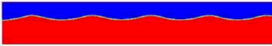
Figure 4. Typical generation of waves in the numerical wave tank ( H=0.05\text{m} , T=2\text{s} ).
