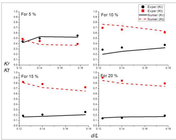
Figure 8. Variation of K_r and K_t with d/L .
