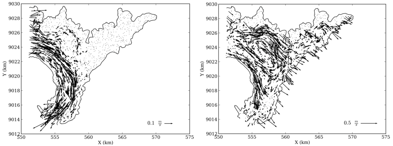
Figure 4. Surface flow simulation for a moderate flood event ( Q_{\max}=4688\text{m}^3\text{s}^{-1} at t=18\text{h} ): flow velocity for the case without wind ( left ) and for extreme wind conditions ( right ).
