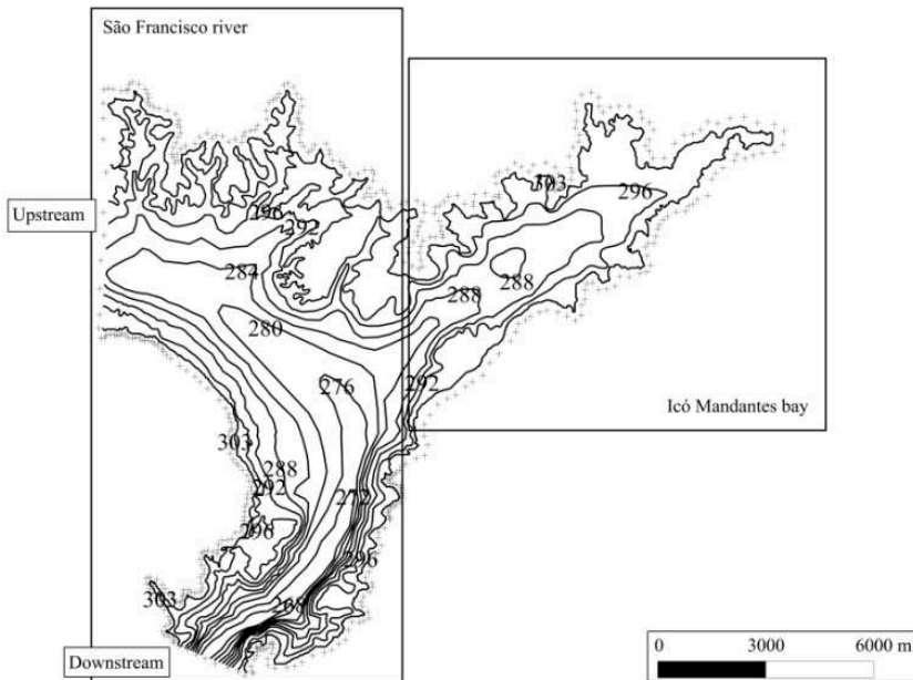
Figure 1. Computational domain of Içó Mandantes bay, Itaparica reservoir.
