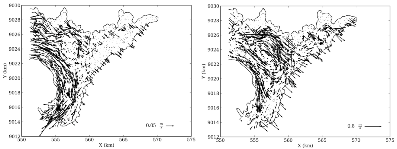
Figure 3. Surface flow simulation for mean flow conditions: flow velocity for mean wind (left) and for extreme wind conditions (right).
