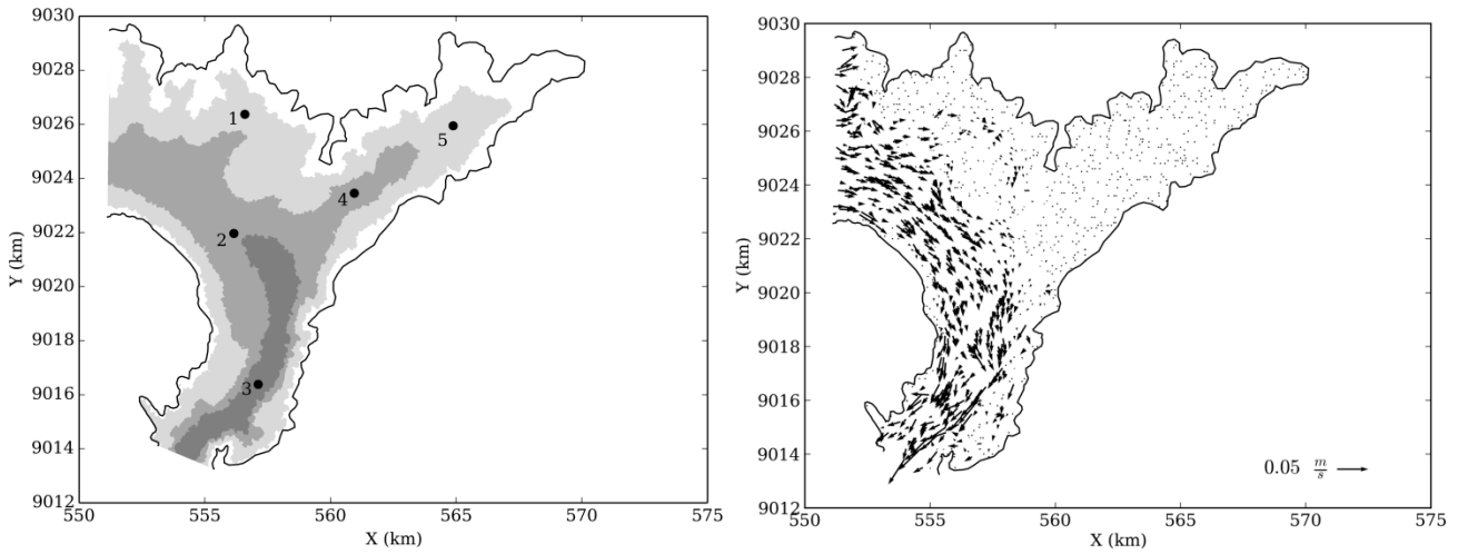
Figure 2. Surface flow simulation for mean flow conditions: control points (left); surface flow simulation without the action of the wind, reference case (right).
