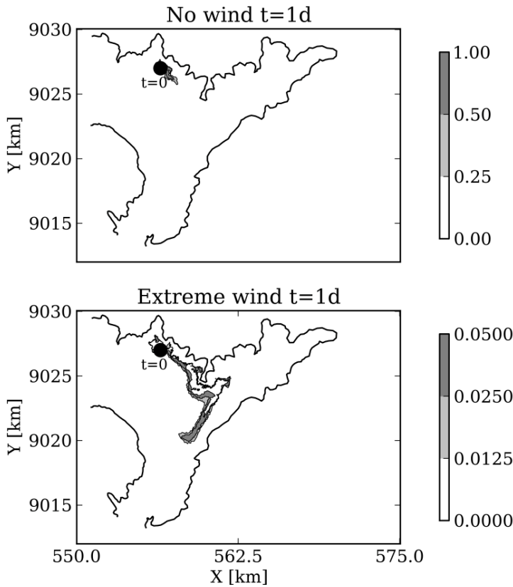
Figure 5. Transport simulation for mean flow conditions: concentration of the tracer for the case without wind ( up ) and for extreme wind conditions ( down ).
