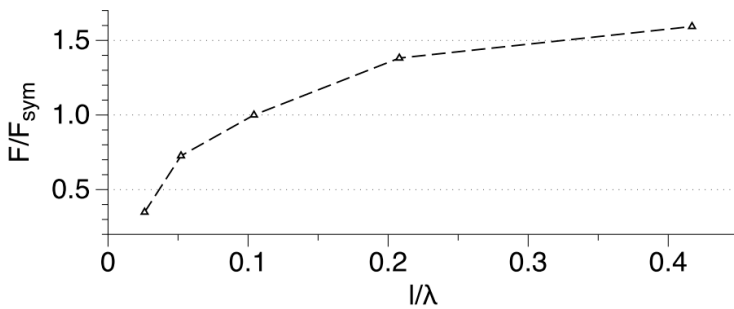
Figure 6. Variation of wave forces with the width l .
