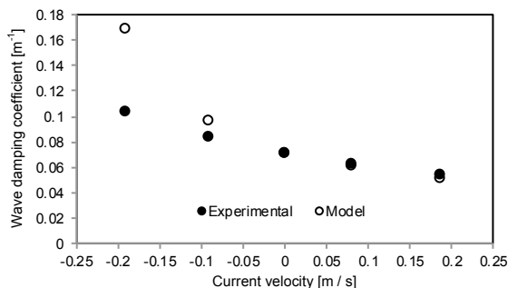
Figure 7. Effect of currents on wave attenuation coefficient on the mud layer.
