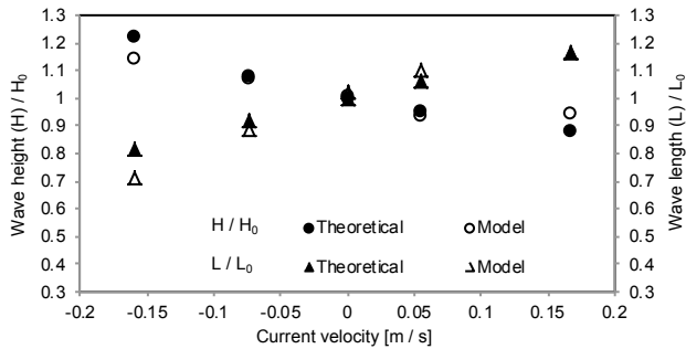
Figure 3. Wave height and wave length variations due to the current on the fixed bed.
