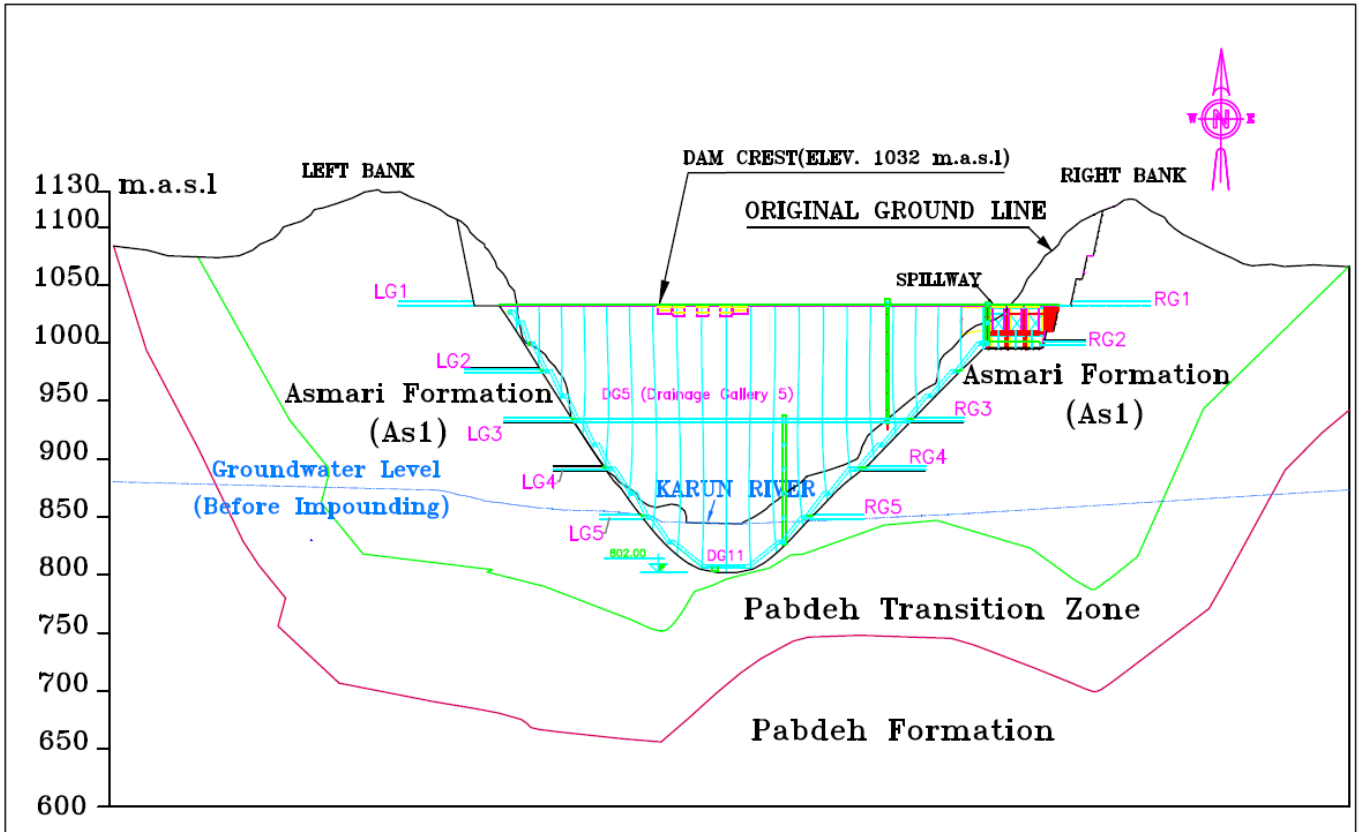
Figure 3. Karun 4 dam geological cross-section viewed from the reservoir downstream towards the dam
