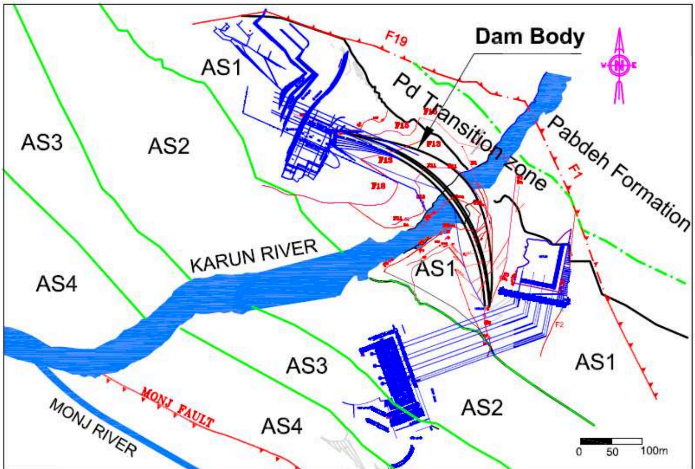
Figure 2. Karun 4 dam geological plan
