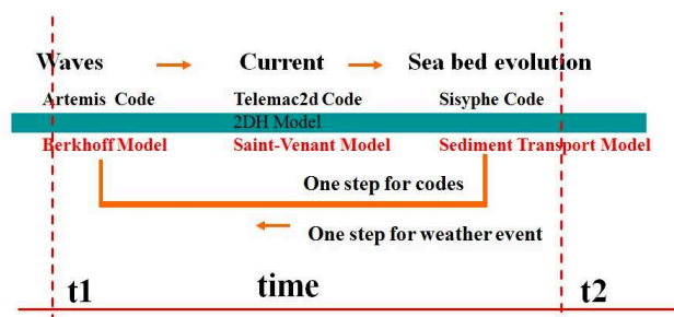
Figure 4. Diagram of the model ATS (Artemis-Telemac-Sisyphé) loop over one weather event time step (between t_1 and t_2 ) used for our simulations.
