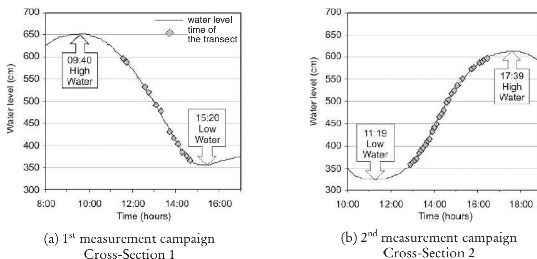
Fig. 4: Time series of water levels and cross-sectional measurements
