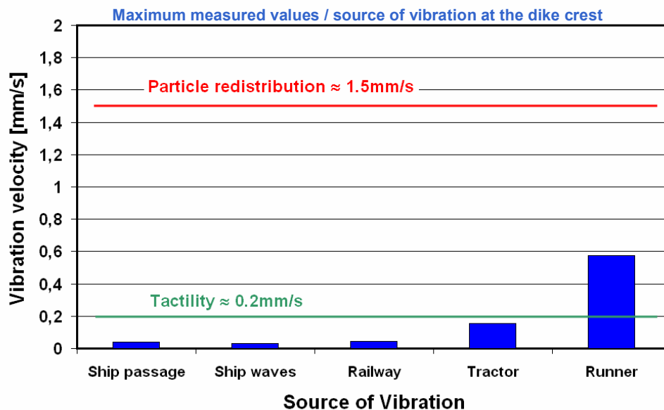
Figure 11. Vibrations of the dike – effect of different sources
