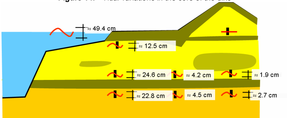
Figure 14. Tidal variations in the core of the dike
