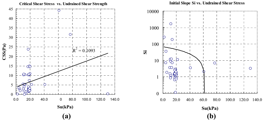
Figure 8: (a) Relationship Between Critical Shear Stress vs. Undrained Shear Strength; (b) Relationship Between Initial Slope S_i vs. Undrained Shear Strength
