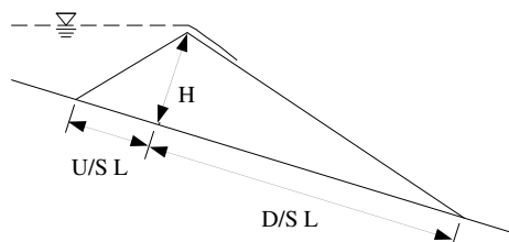
Fig. 4 Shape and size of the dam body
