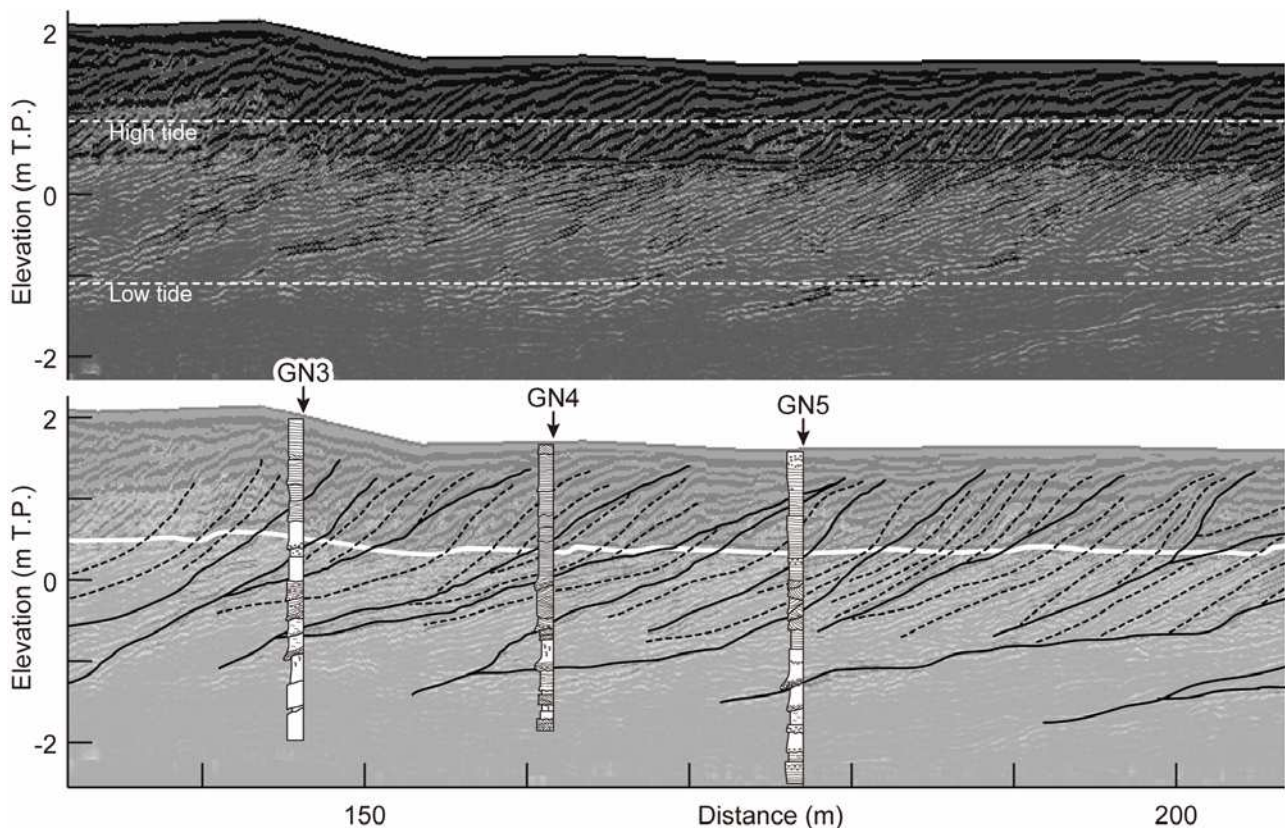
Fig.5 GPR Profiles and columner sections of sediment cores.
